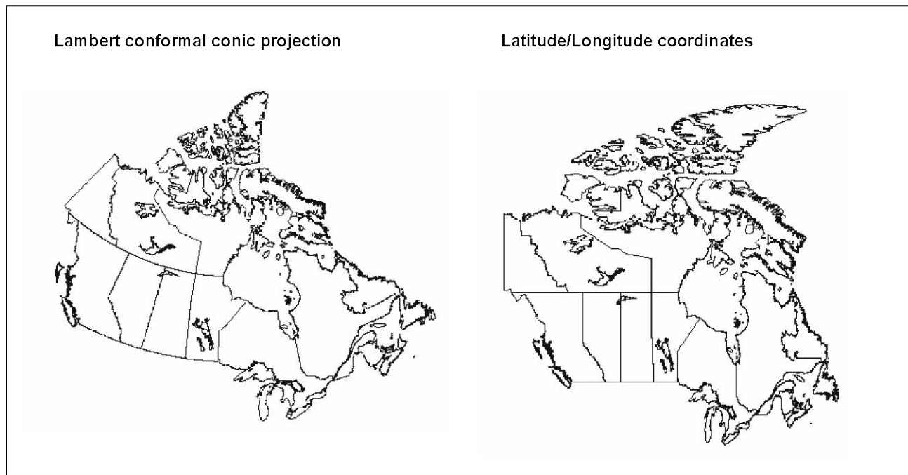
Figure 2.2 Example of a map projection and unprojected coordinates
