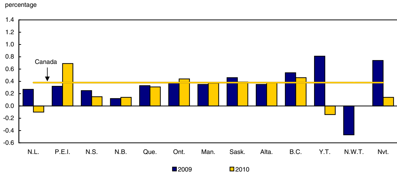
Chart 2 Quarterly variation of population estimates, Canada, provinces and territories, July to September, 2009 and 2010
