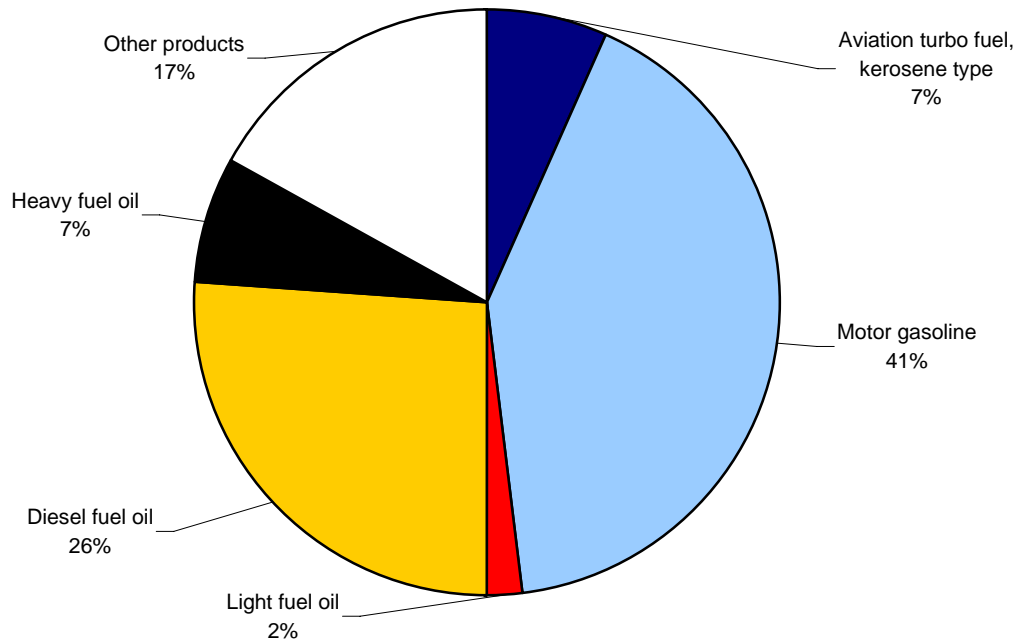
Domestic sales of refined petroleum products - by product - August 2005
