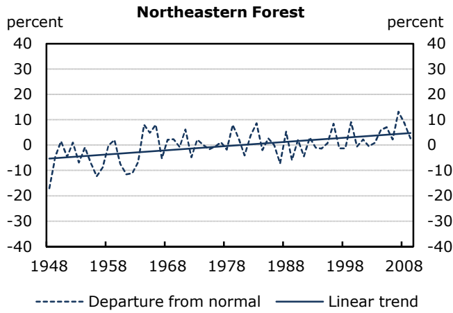
Chart 2 Annual mean precipitation percentage departures from 1961 to 1990 normal and linear trend for climatic regions, 1 1948 to 2009
