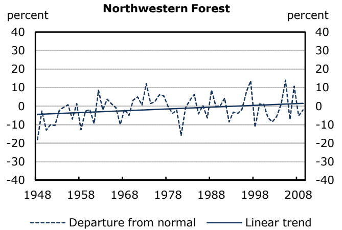
Chart 2 Annual mean precipitation percentage departures from 1961 to 1990 normal and linear trend for climatic regions, 1 1948 to 2009
