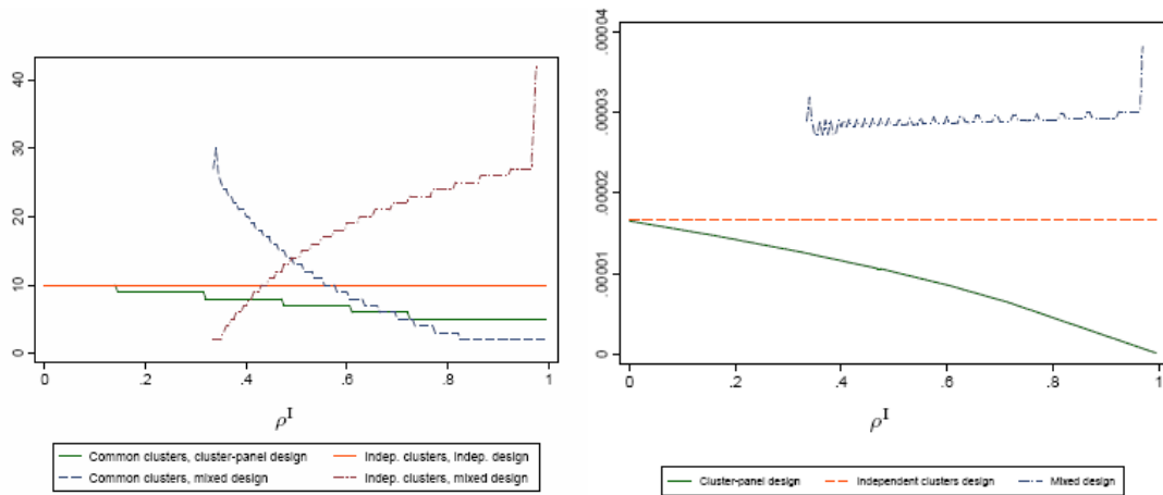
Figure 1: Number of clusters and Vd[\bar{y}^{(2)} - \bar{y}^{(1)}] as a function of \rho^I .
